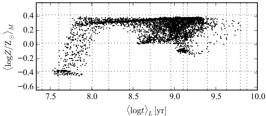
NGC2663 T007
