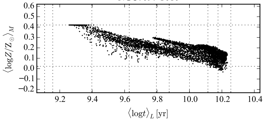
NGC7097 T010
