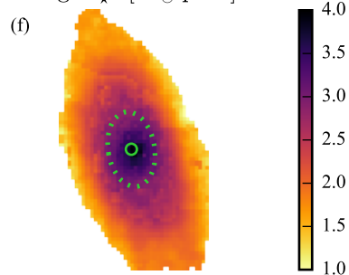
b^{\text{gal}}
