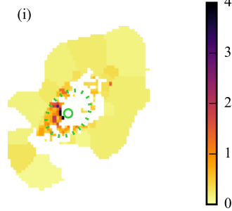
\sigma_{\star} [\text{km s}^{-1}]
