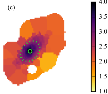
\log \Sigma_{\star}^{\text{dez}} [M_{\odot} \text{pc}^{-2}]
