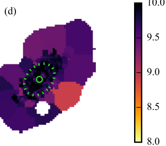
\log \Sigma_{\text{SFR}} [M_{\odot} \text{Gyr}^{-1} \text{pc}^{-2}]
