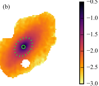
\langle \log Z \rangle_M [Z_{\odot}]
