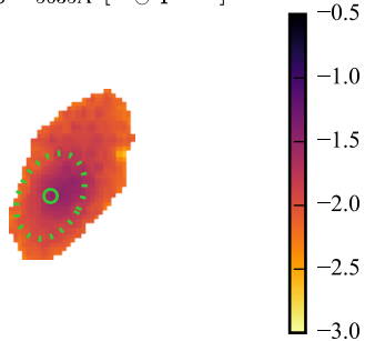
\langle \log Z \rangle_M [ Z_{\odot} ]
