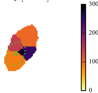
\sigma_{\star} [ \text{km s}^{-1} ]
