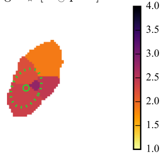
\log \Sigma_{\star}^{\text{dez}} [ M_{\odot} \text{pc}^{-2} ]
