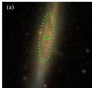
\langle \log t \rangle_{\text{L}} [\text{yr}]
