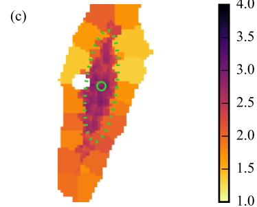
\log \Sigma_{\star}^{\text{dez}} [\text{M}_{\odot} \text{pc}^{-2}]
