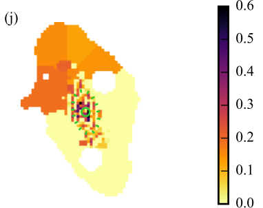
\tau_V
