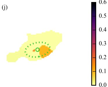
\tau_V
