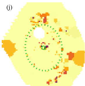
\tau_V
