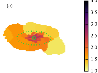
\log \Sigma_{\star}^{\text{dez}} [\text{M}_{\odot} \text{pc}^{-2}]
