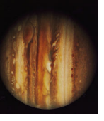
Left: An artistic representation of Jupiter's atmosphere, by Don Dixon.
