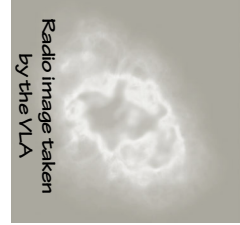
Radio image taken by the VLA
