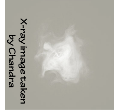
X-ray image taken by Chandra
