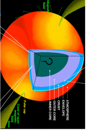
Anatomy of a neutron star as pictured by Dany Page (Univ. of Mexico)
