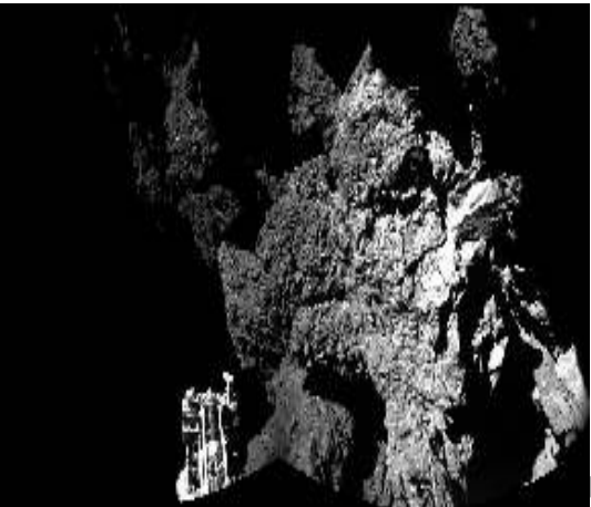
The Philae lander in 2014 after being dropped off on comet 67P/Churyumov-Gerasimenko by the Rosetta probe after a 10-year journey (Credit ESA).
