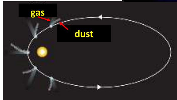
Direction of the tails of a comet according to its position relative to the Sun. They are always opposite to the Sun.
