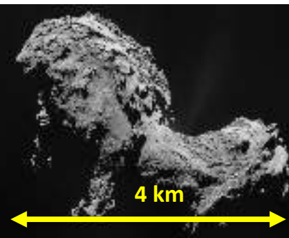
The nucleus of comet 67P/Churumov-Guerassimenko taken by the Rosetta probe in September 2014. (ESA)
