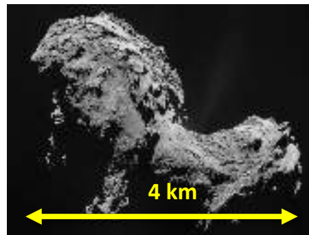
The nucleus of comet 67P/Churumov-Guerassimenko taken by the Rosetta probe in September 2014. (ESA)
