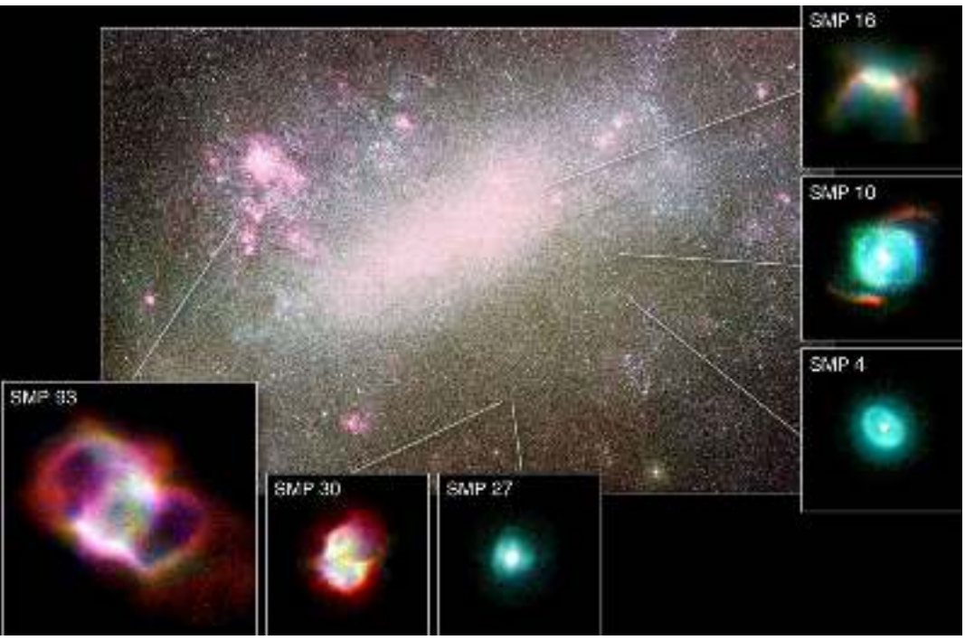
The Large Magellanic Cloud and the positions of a few planetary nebulae of various morphologies. 10
