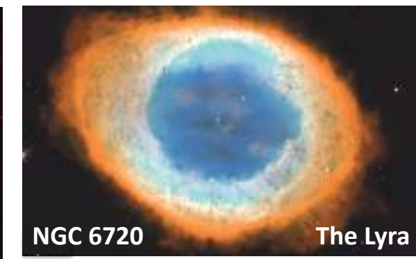
Two of the most famous planetary nebulae (Source HST)
