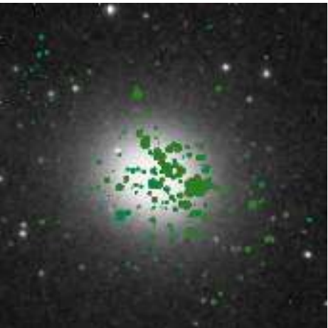
The elliptical galaxy NGC 3379. The green dots mark the positions of planetary nebulae detected by the PN.spectrograph. Measurement of their radial velocities
