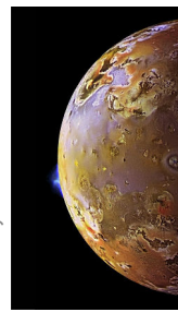
Artist's rendition of Io, with some of its volcanoes erupting. (SwRI/Andrew Blanchard/NASA)
