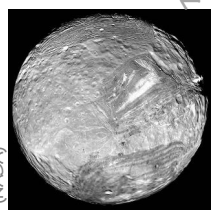
Miranda, one of Uranus' satellites. (NASA/JPL)
