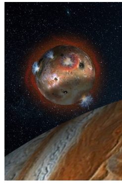
Artist's rendition of Io, with some of its volcanoes erupting. (SwRI/Andrew Blanchard/NASA)
