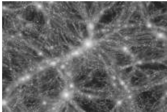
Simulation of the cosmic web
