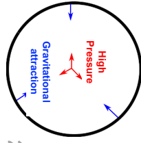
A star is in equilibrium between the outward action of thermal pressure and the inward action of gravity .
