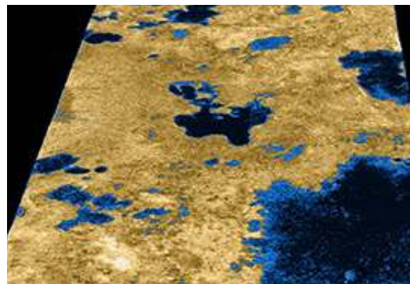
Lakes of hydrocarbons, methane and ethane on Saturn's satellite Titan.
