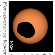
A transit of Phobos, one of the moons of Mars, as seen from the surface of Mars. The shadow is not round because Phobos is not spherical. The Perseverance Rover, a robotic rover exploring the planet Mars.
