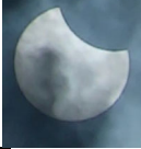
When the Moon passes in front of the Sun, a solar eclipse occurs. Here is a picture of a partial eclipse.
