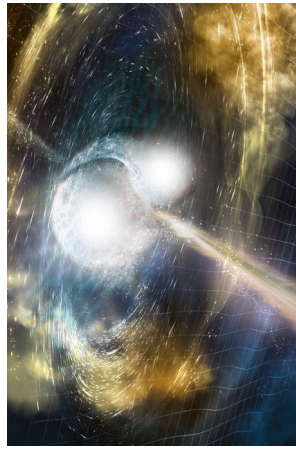
An artist's depiction of two merging neutron stars. The narrow beams are the gamma-ray bursts. Swirling clouds of material ejected from the merging stars are also shown. These clouds emit in visible light as well as other wavelengths.
