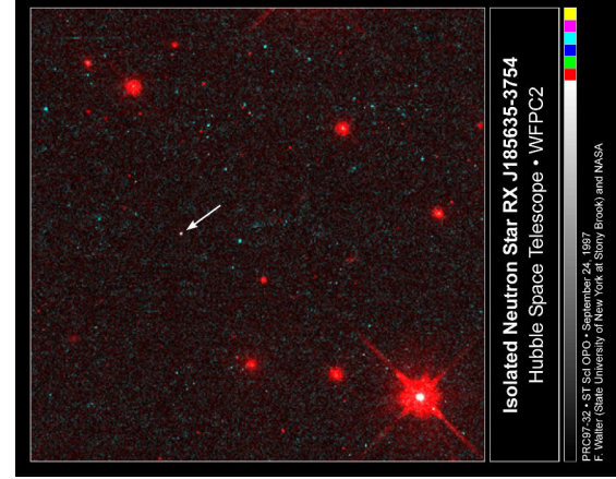
This image shows how a nearby neutron star looks like from Earth, in visible light.
