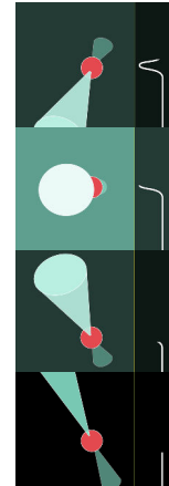
The majority of known neutron stars are radio pulsars rotating about their axes. The beam they emit is detected by radio antennae when the beam is directed towards the Earth.
