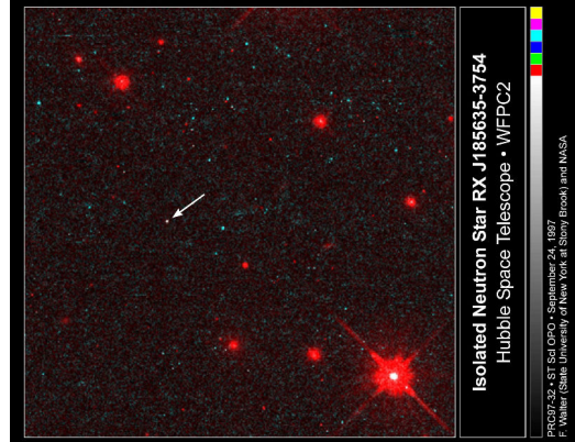
Isolated Neutron Star RX J185635-3754 Hubble Space Telescope • WFPC2 PRC07-29 • ST ScD DPO • September 24, 1997 F. Walter (State University of New York at Stony Brook) and NASA
