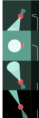
The majority of known neutron stars are radio pulsars rotating about their axes. The beam they emit is detected by radio antennae when the beam is directed towards the Earth.
