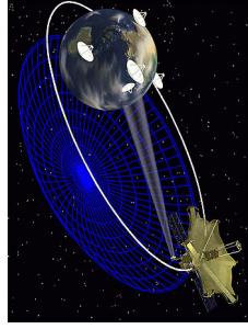
as the telescopes on the ground. The resolution is that of an equivalent radio telescope larger than the Earth (represented in blue in the figure) but the collecting surface remains very small, so only very bright objects can be observed.
