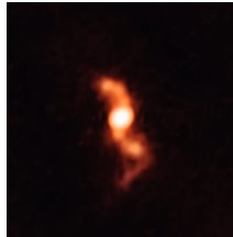
Object SS 433, microwave image, Credit: ALMA (ESO/NAOJ/NRAO)/K. Blundell (University of Oxford, UK), R. Laing, S. Lee & A. Richards, Ap J Letters.
